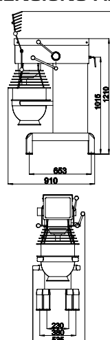
DIMENSIONS AR40
