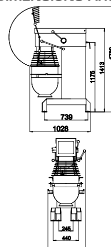
DIMENSIONS AR60
