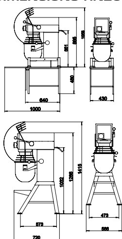
DIMENSIONS RN20
