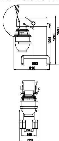
DIMENSIONS AR30
